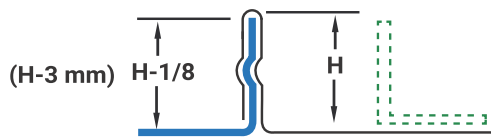
STANDING SEAM T-15
