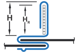
STANDING S (BAR REINFORCED) T-13
