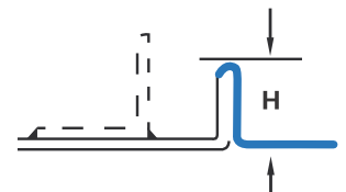
T-21 WELDED FLANGE (T-21a REINFORCED W.F.)
