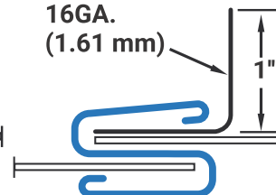
REINFORCED "S" SLIP T-7
