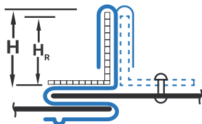
STANDING S (ANGLE REINFORCED) T-14
